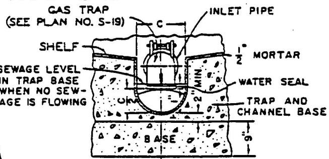
SECTION X-X
