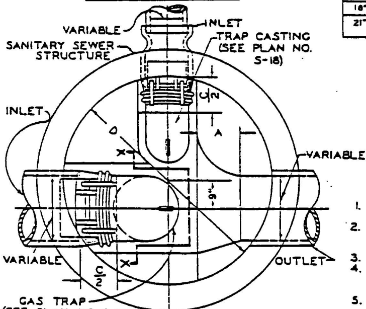
PLAN DOUBLE TRAP BASE
