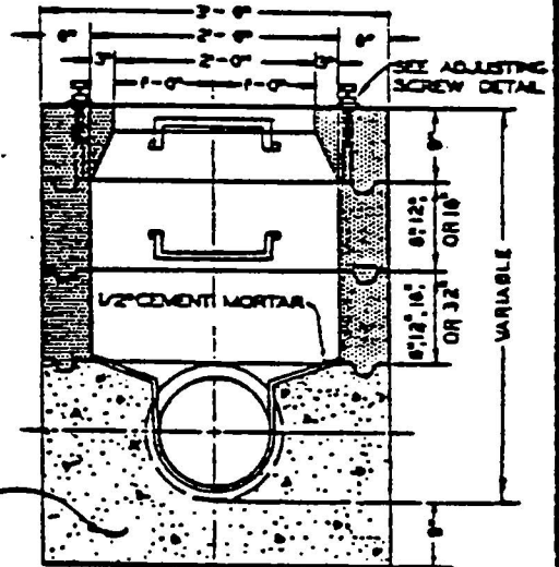
SECTION B-B TYPE B
