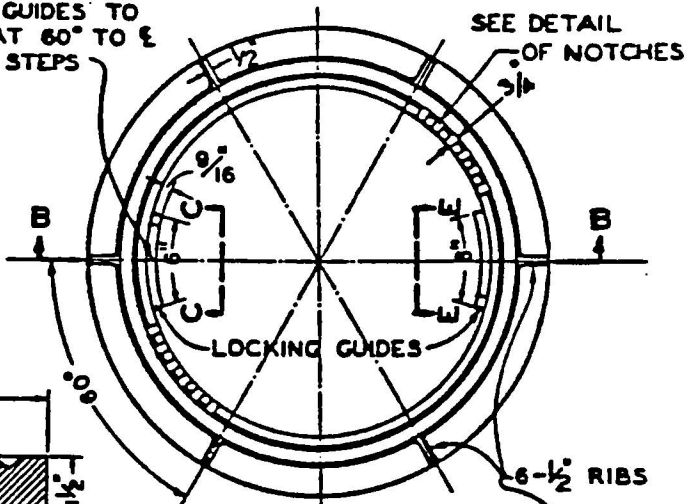
PLAN OF FRAME
