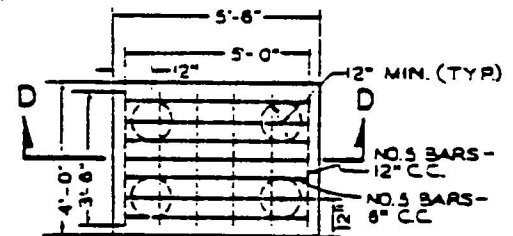
PRECAST CONCRETE SHALLOW BASE
