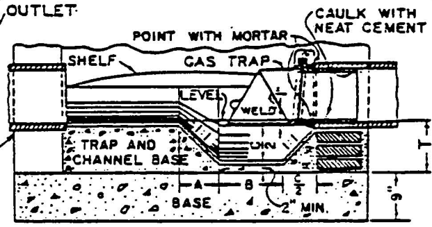
SECTION Y-Y
