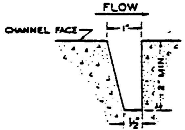
CROSS SECTION OF NOTCH SIDES AND BOTTOM
