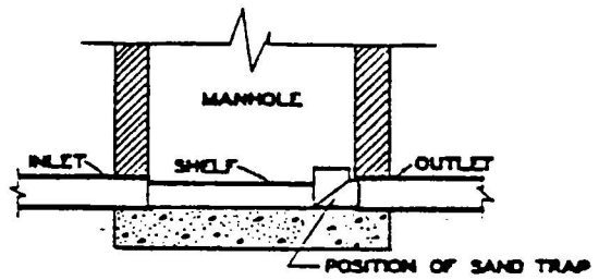
SECTIONAL VIEW SHOWING PLACEMENT OF SAND TRAP
