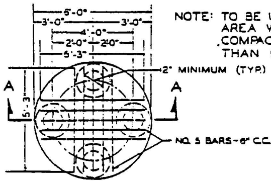
ROUND BASE
