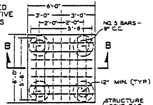
SQUARE BASE
