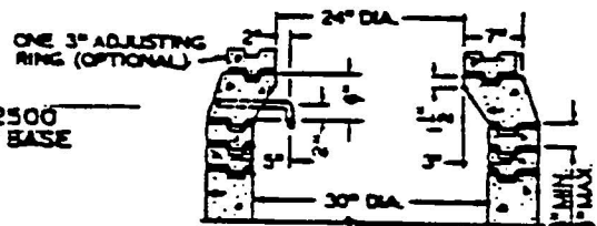
REDUCER RING AND ADJUSTING RINGS
