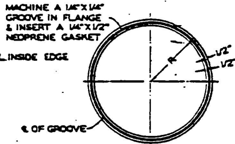
FLANGE FACE (STUB CASTING)
